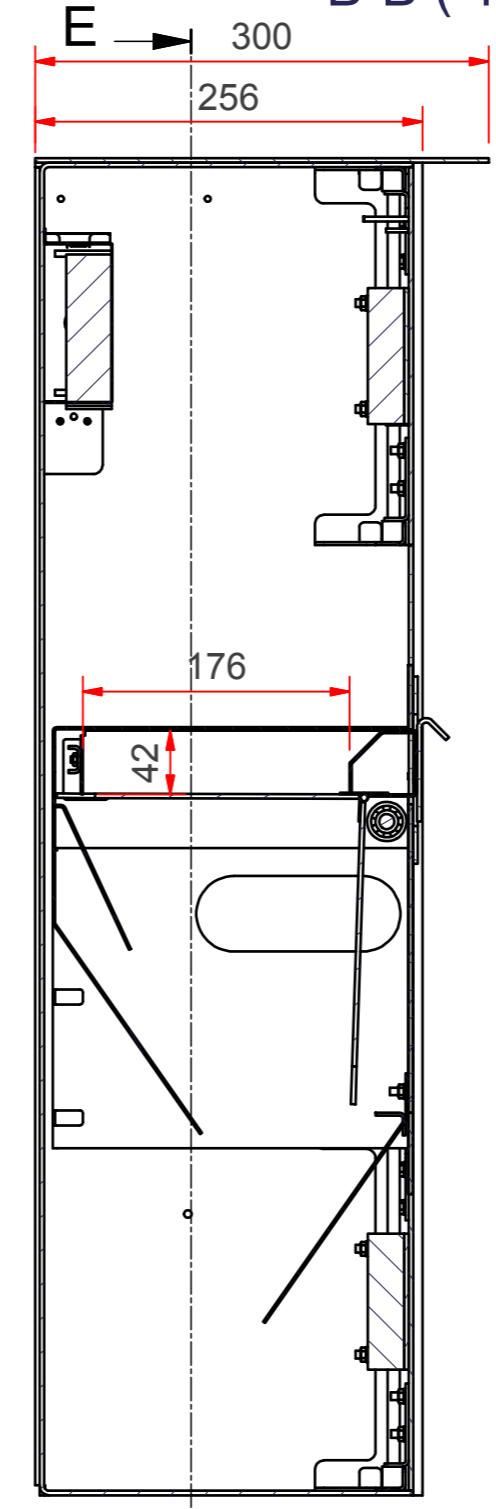
B-B (1:5)
